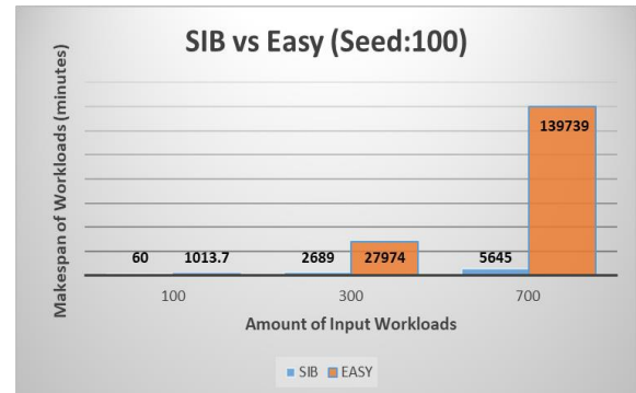
Fig. 2(b). SIB versus EASY at 100 seeds.
