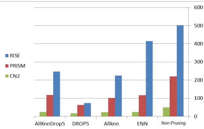
Fig. 4. Comparing the average number of generated rules before and after applying instance reduction methods for different rule induction.
